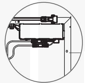
Attached Micro-inverter
