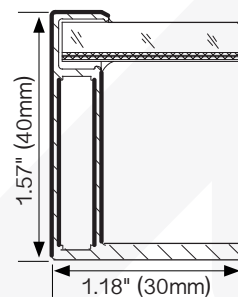
Frame Cross-Section
