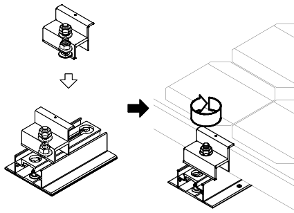
Middle Clamp
