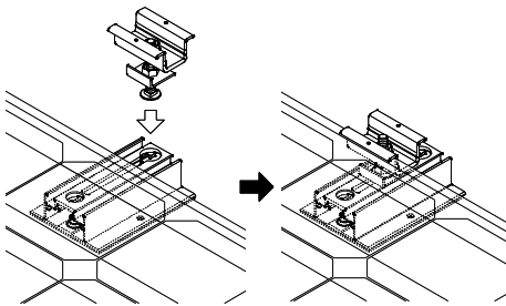
Middle Clamp
