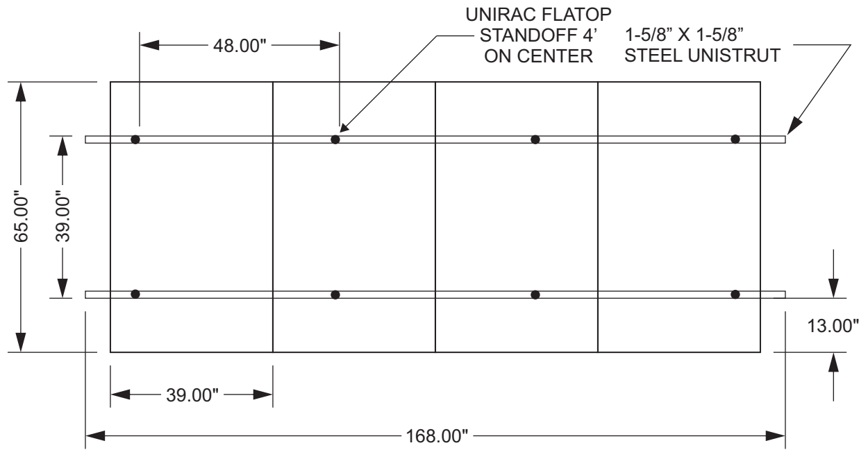
MAGE 250W / 6PL SOLAR PANEL (TYPICAL 4)
