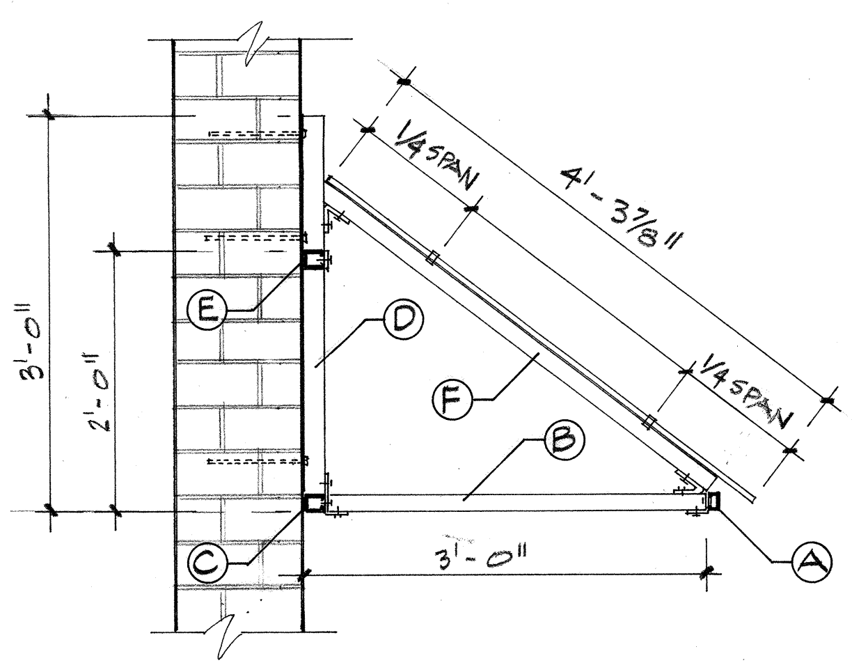
CROSS SECTION 1" = 1'-0" SCALE
